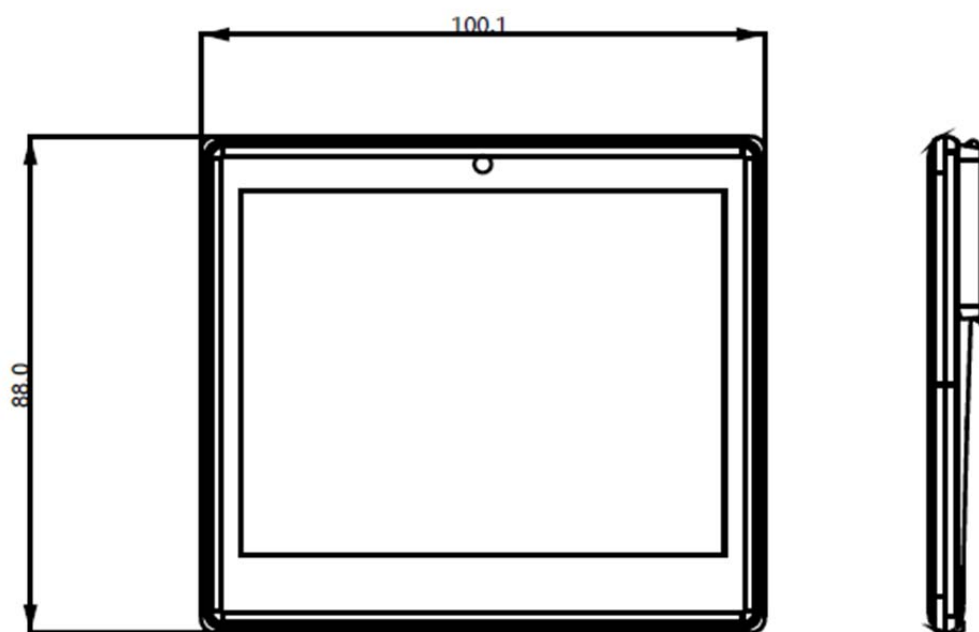
Figure 2-10 4.2" dimension
