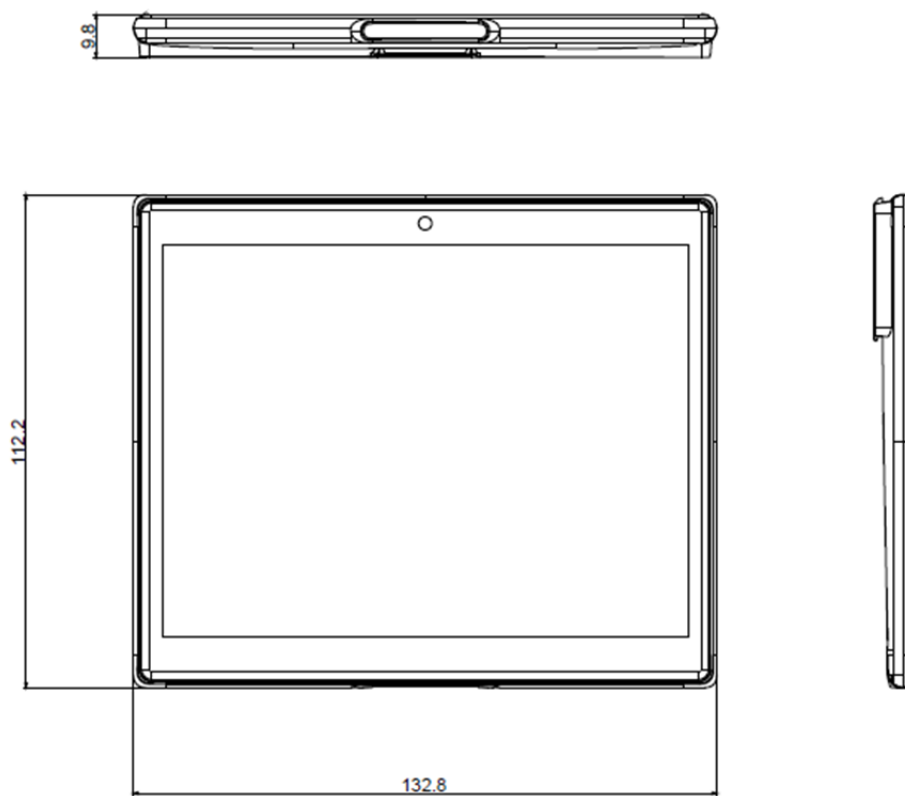
Figure 2-111 5.83" dimension
