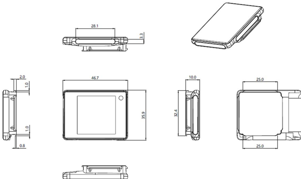
Figure 2-3 1.54" dimension
