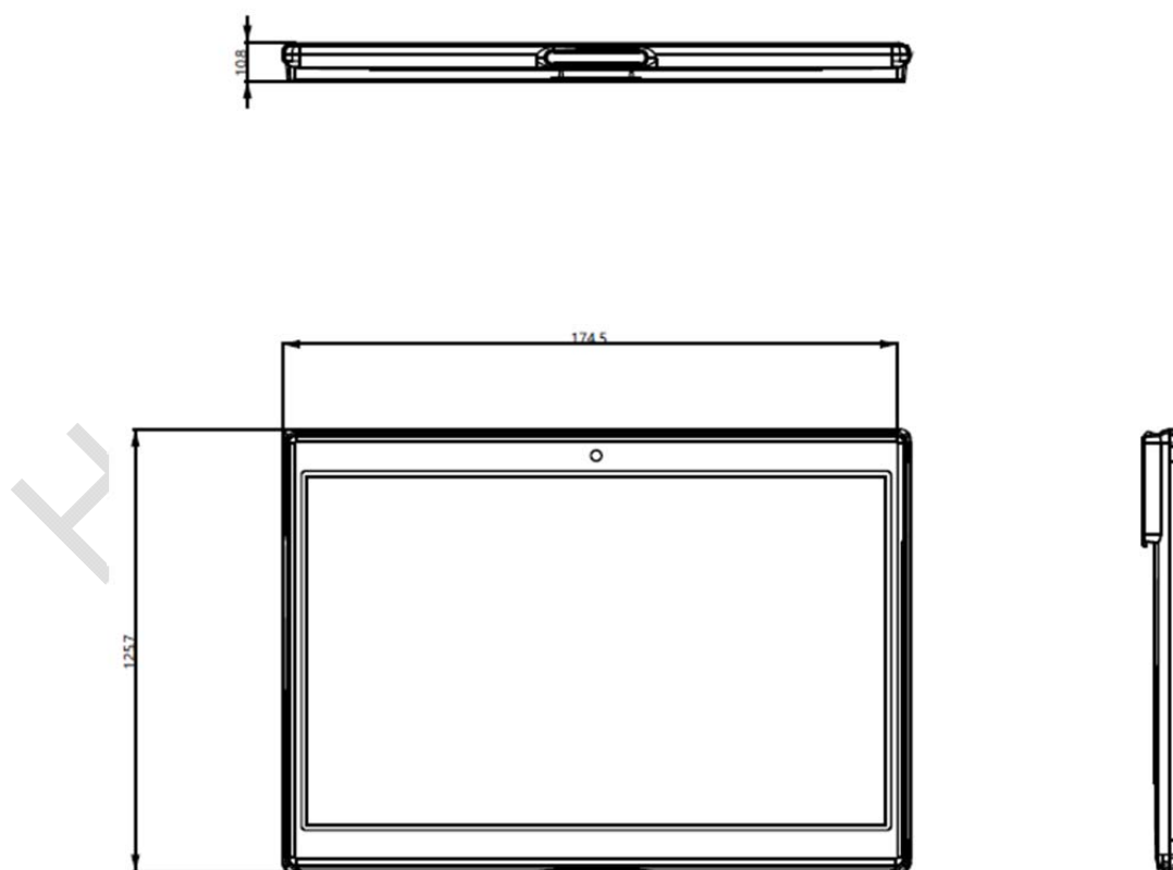
Figure 2-12 7.5" dimension
