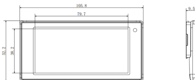
Figure 2-9 3.5" dimension
