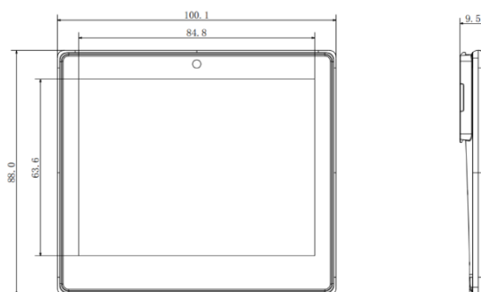
Figure 2-10 4.2" dimension
