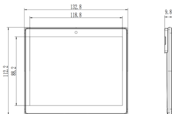
Figure 2-11 4.37" dimension
