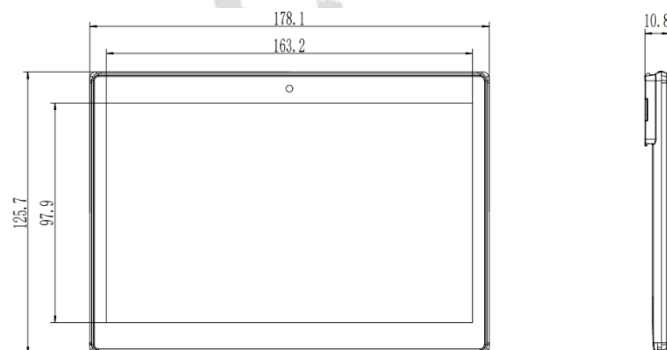
Figure 2-12 5.83" dimension
