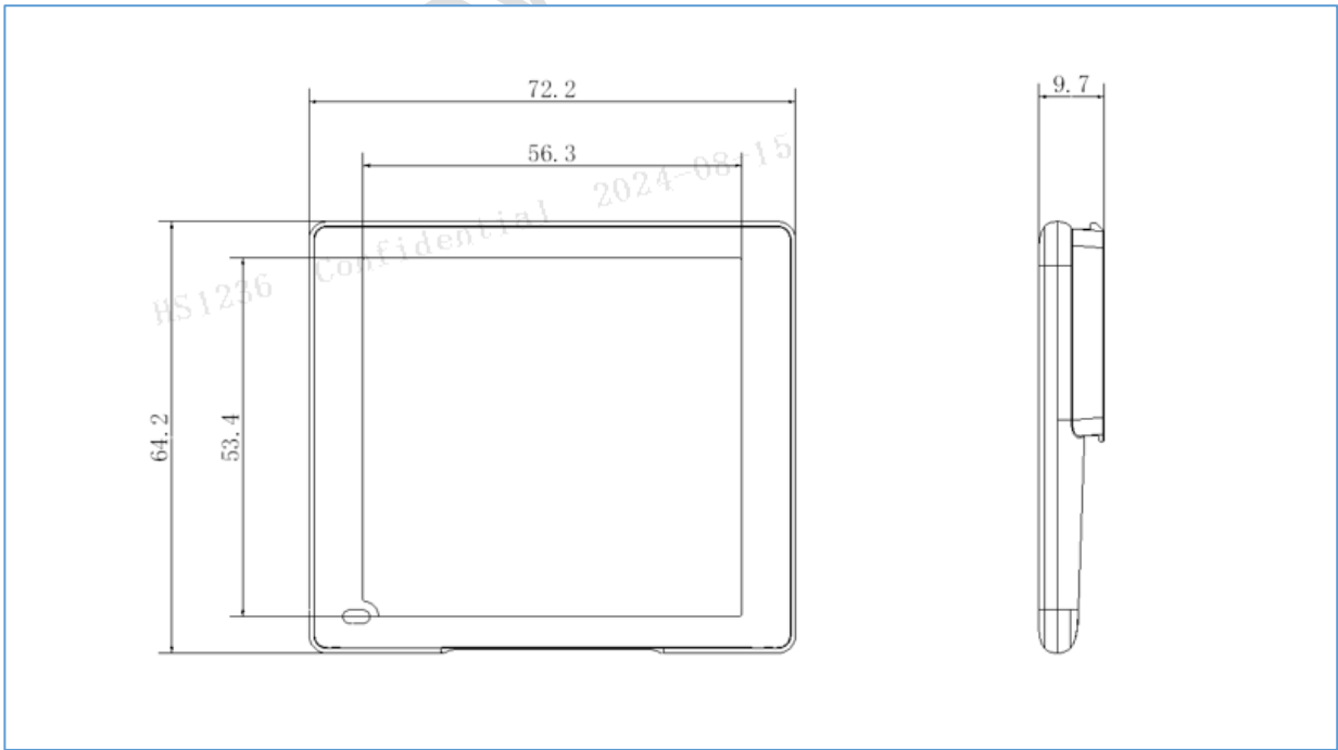
Figure 2-8 3.1" dimensions
