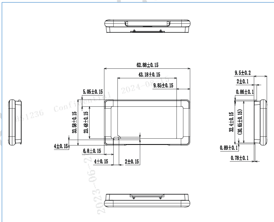
Figure 2-4 2.0" dimensions
