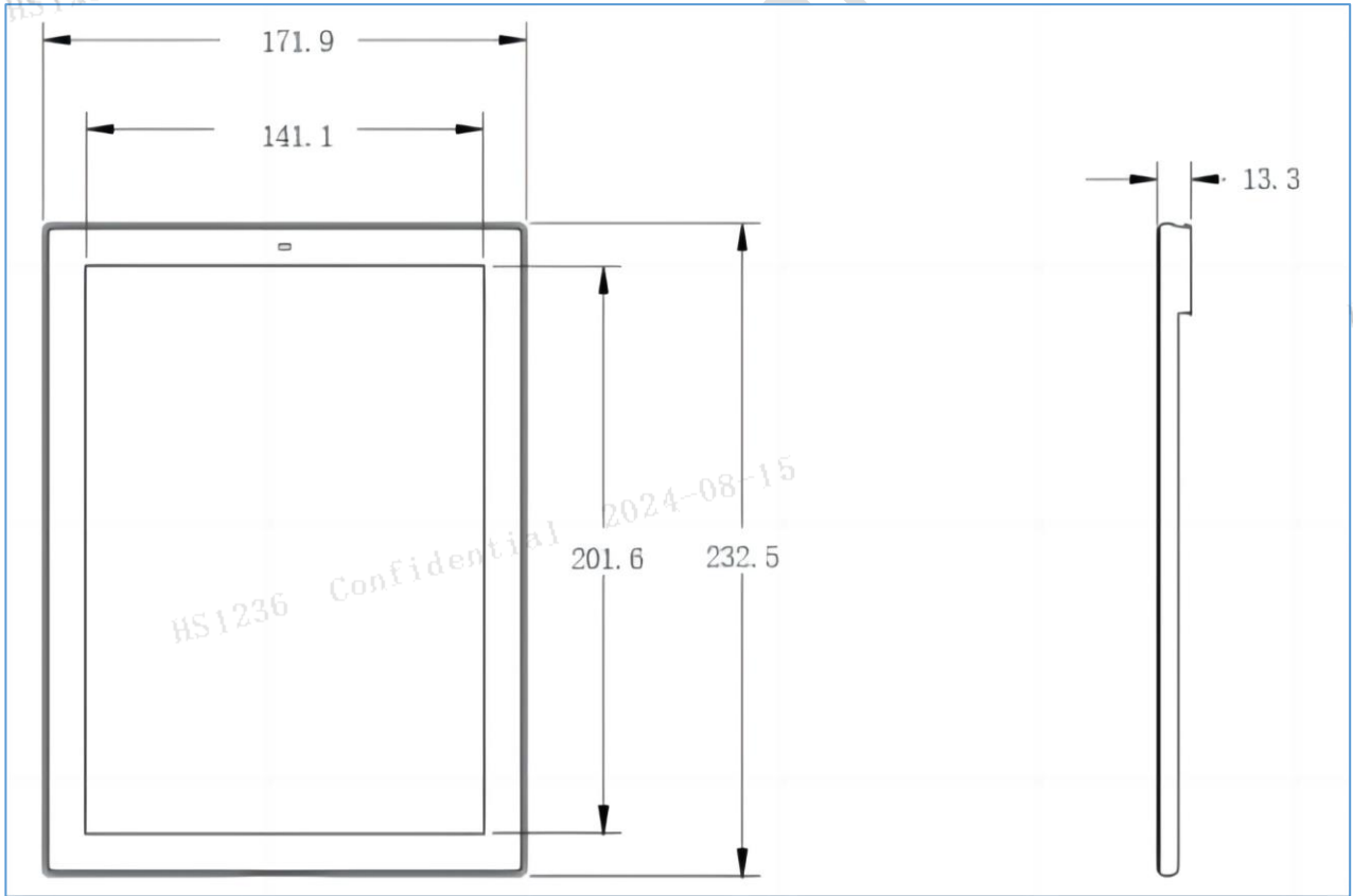
Figure 2-12 9.7” dimensions
