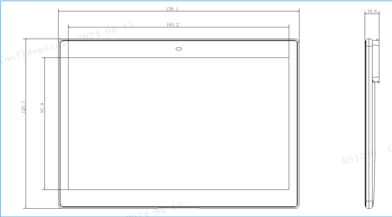
Figure 2-11 7.5” dimensions
