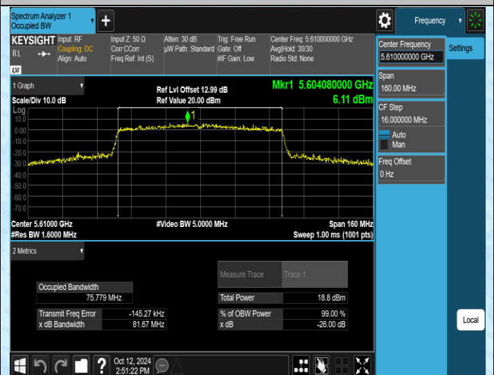
11AC80MIMO-Ant2-5610
