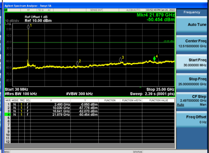
Mode 1 / CH39(2480MHz)
