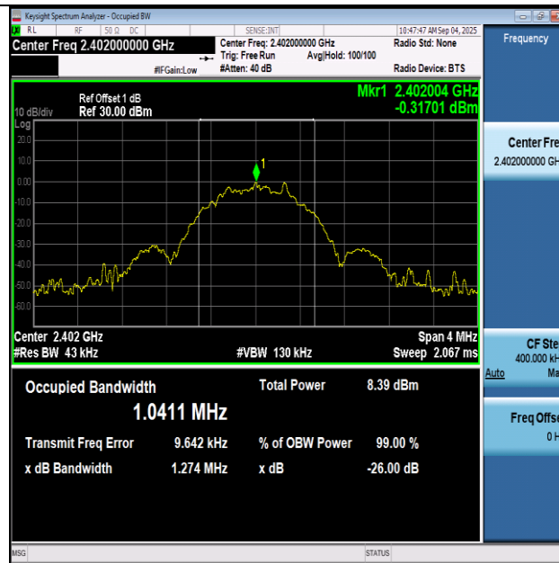
BLE_1M-Ant1-2402
