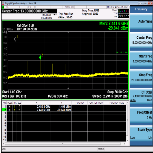
BLE_2M-Ant1-2480-1000~25000-PASS
