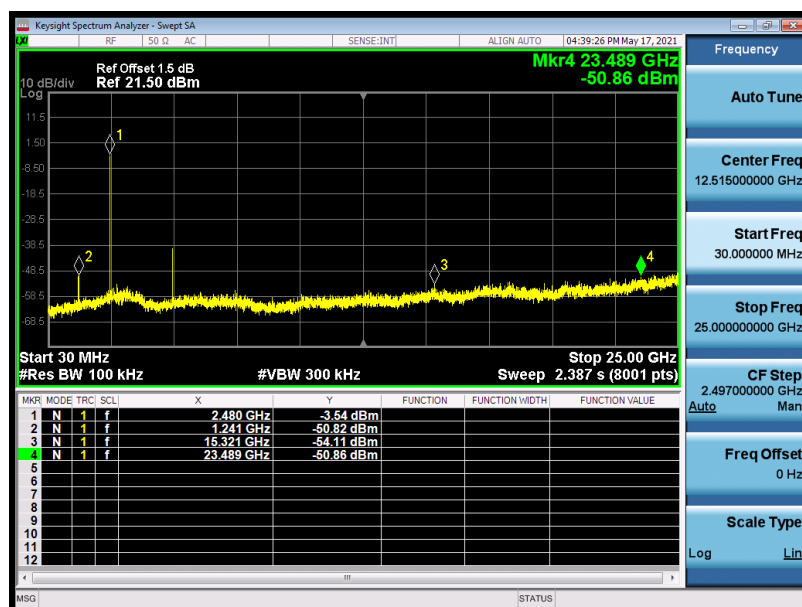
Mode 1 / CH39(2480MHz)
