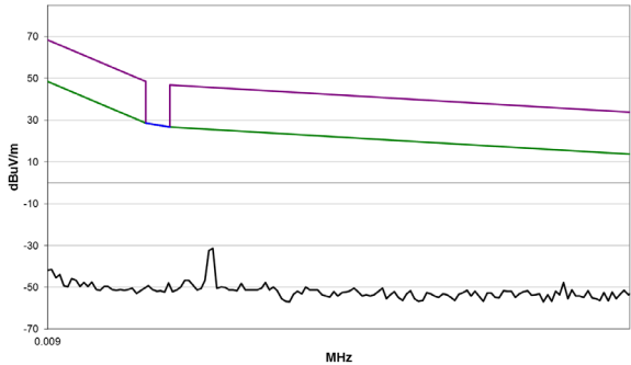
9 kHz to 490 kHz
