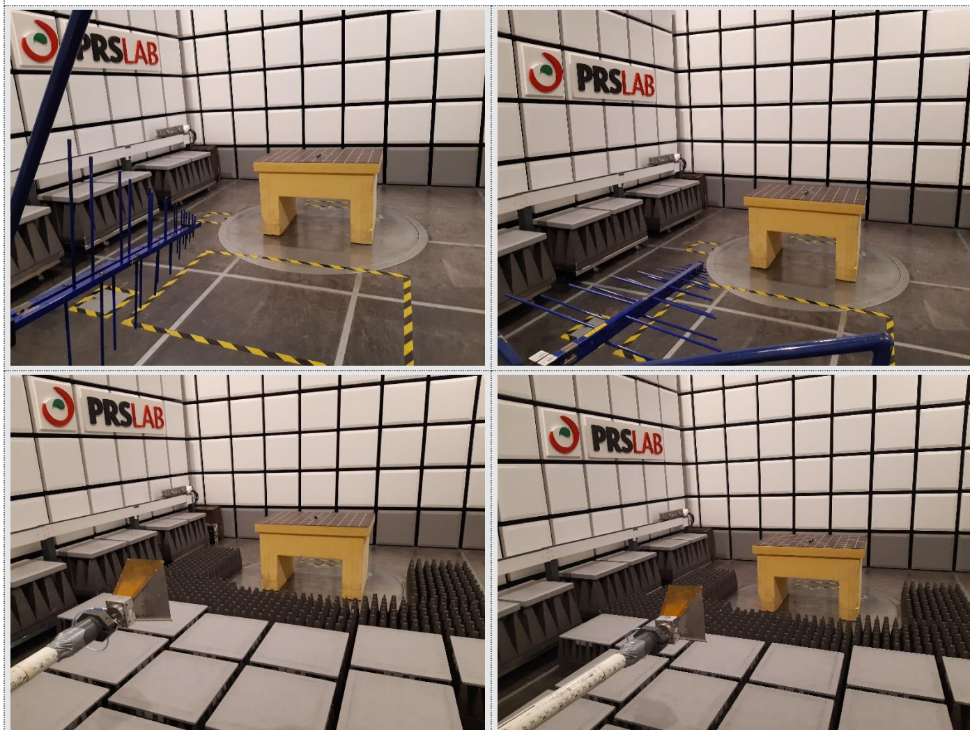
PHOTO N° 2 - RADIATED EMISSIONS SETUP
