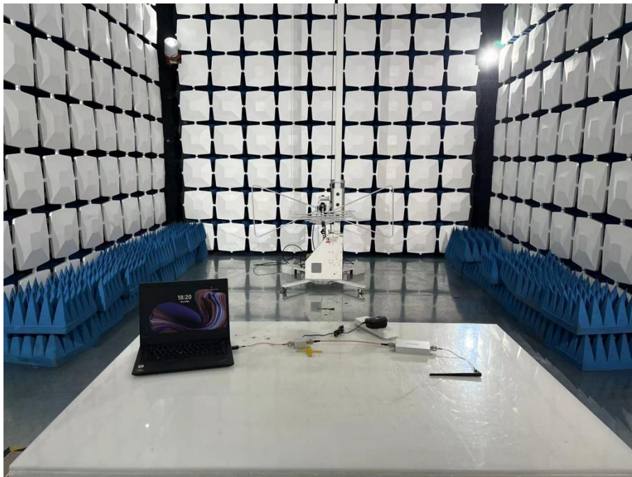
Radiated Emission Test Setup Photo - Below 1GHz 192
