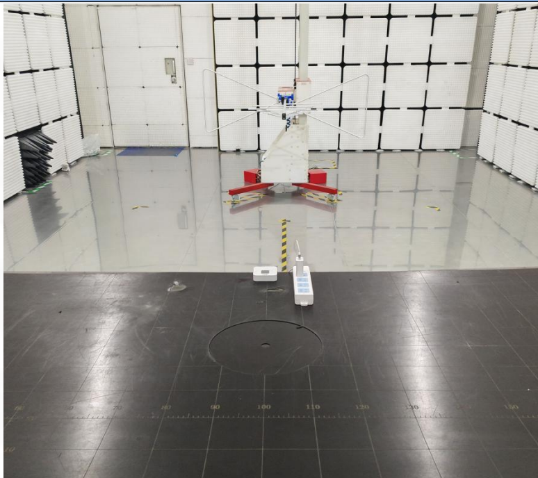
Emissions in restricted frequency bands (below 1GHz)
