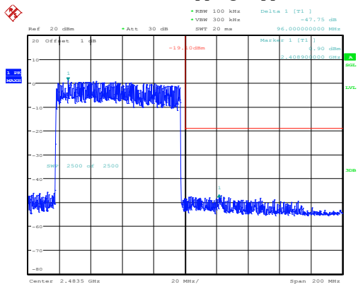
3DH1_Hopping_Upper
