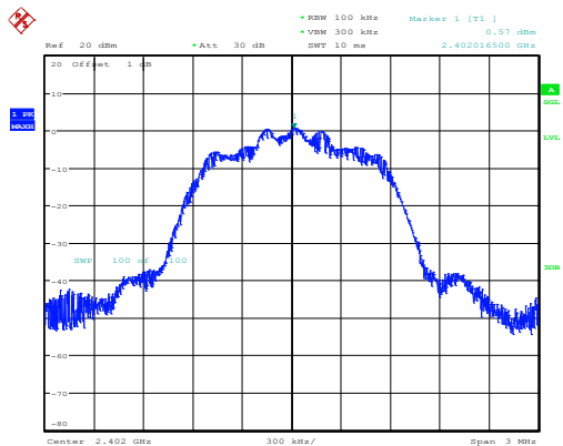
3DH1_Low
