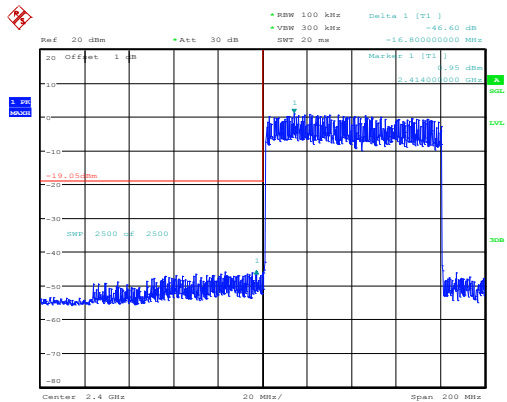
2DH1_Hopping_Lower
