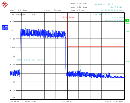
2DH1_Hopping_Upper
