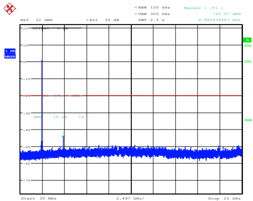
3DH1_Middle
