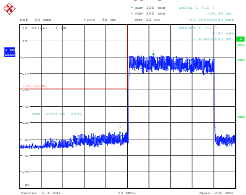
3DH1_Hopping_Lower
