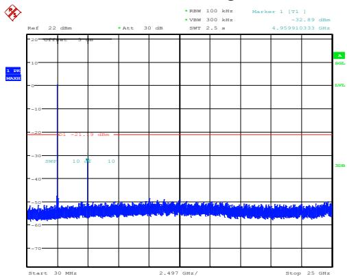
3DH1_High
