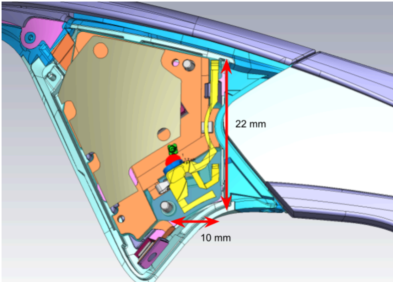
Antenna Photo:
