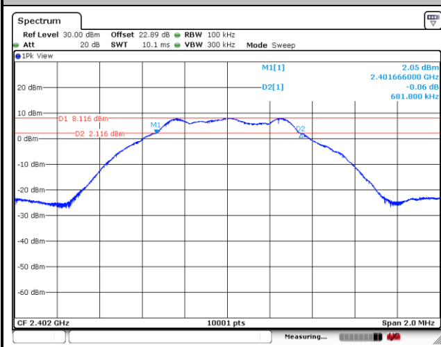
6 dB Bandwidth Plot on Channel 0
