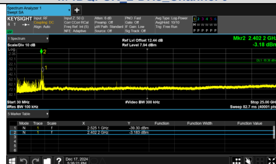
30.0 MHz - 25000.0 MHz π/4DQPSK 2-DH5 Channel 0
