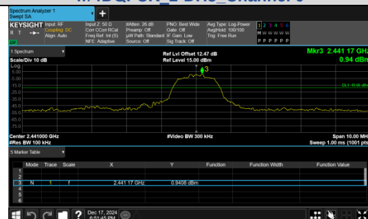
Out Of Band Emission \pi/4 DQPSK 2-DH5 Channel 39
