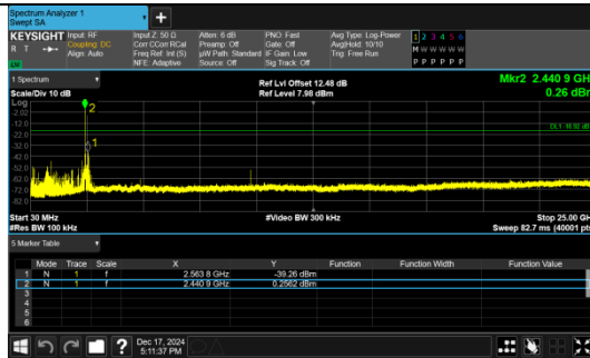
30.0 MHz - 25000.0 MHz GFSK_DH5_Channel 39
