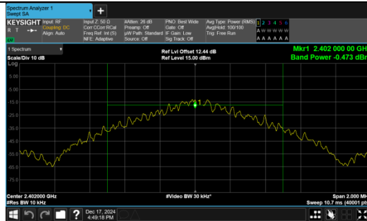
Average Output Power GFSK Channel 0
