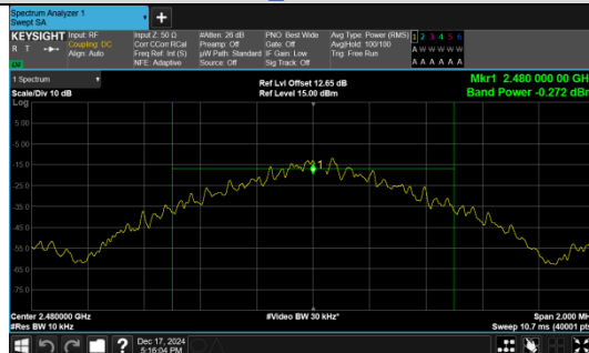
Average Output Power GFSK Channel 78
