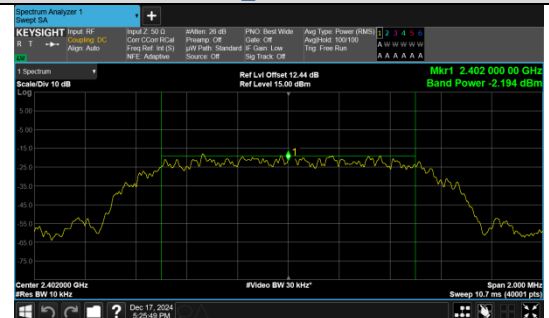
Average Output Power \pi/4 DQPSK Channel 0
