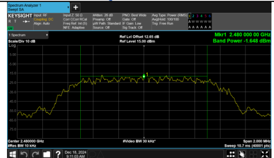
Average Output Power \pi/4 DQPSK Channel 78
