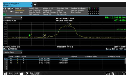
Out Of Band Emission \pi/4 DQPSK 2-DH5 Channel 0
