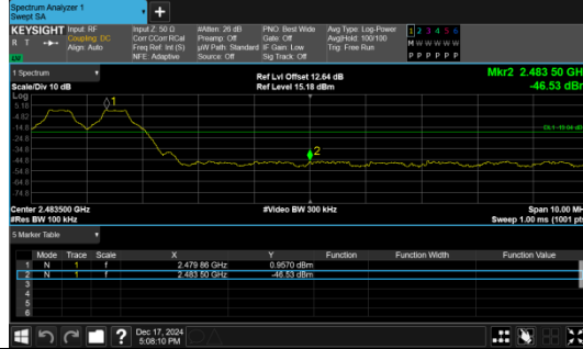
Out Of Band Emission(Right) GFSK DH5 Channel Hopping
