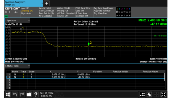
Out Of Band Emission(Right) \pi/4 DQPSK 2-DH5 Channel Hopping
