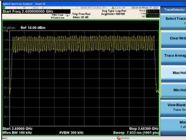
8DPSK Modulation
