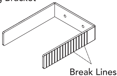
Mounting Bracket
