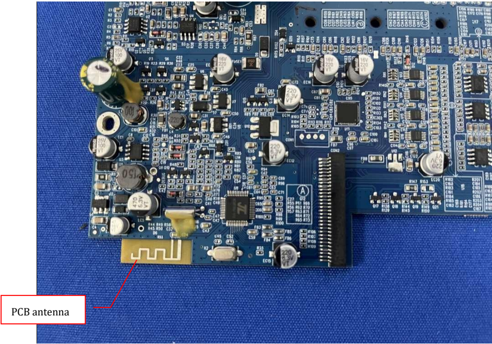
EUT Internal View 3
