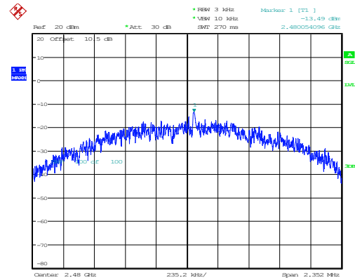
BLE_2M_High_Channel
