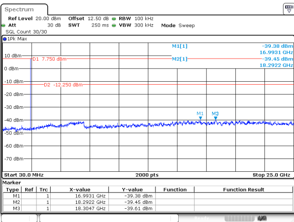
BLE_1M_Middle_Channel
