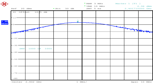
Low channel 2.96dBm
