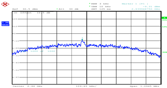
Middle channel -9.31dBm/3kHz
