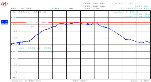
Low channel 0.731MHz
