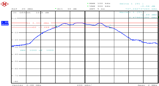
High channel 0.737MHz
