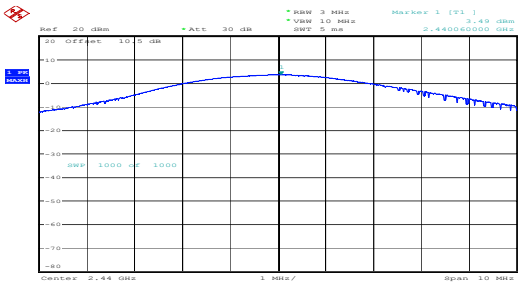
Middle channel 3.49dBm
