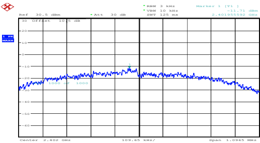
Low channel -11.71dBm/3kHz
