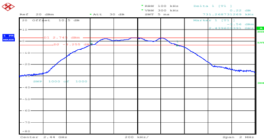
Middle channel 0.731MHz
