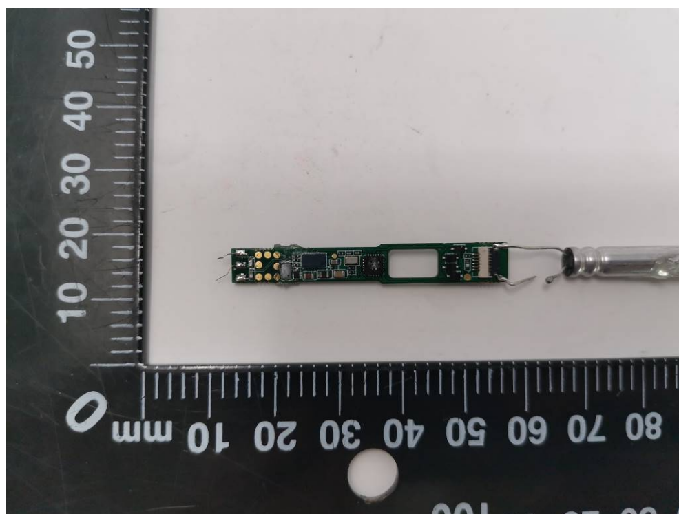
Fig.4 PCB view-02
