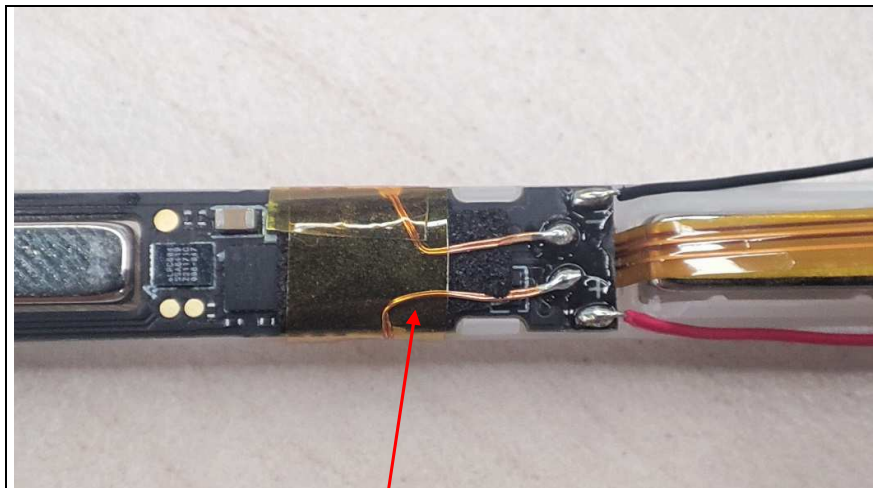
Coil for wireless charging
