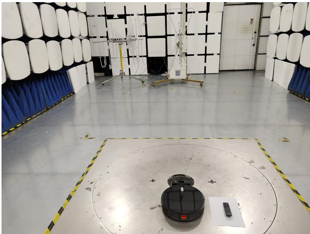
Below 1 GHz
