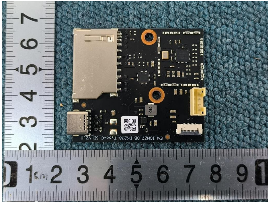
SECONDARY BOARD 3 TOP VIEW (WITHOUT SHIELDING)
