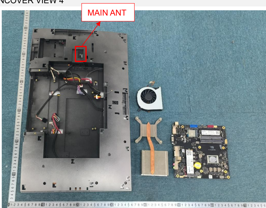
EUT UNCOVER VIEW 4
