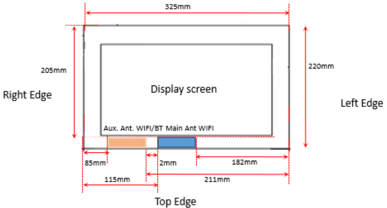
Main Antenna
