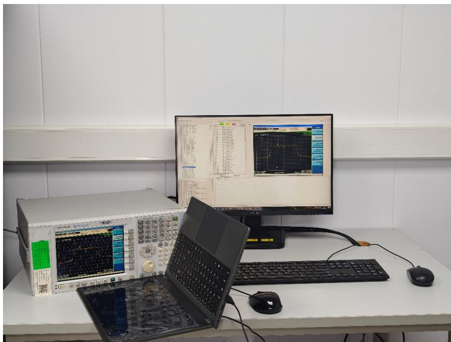
Conducted Test-BT/WIFI
