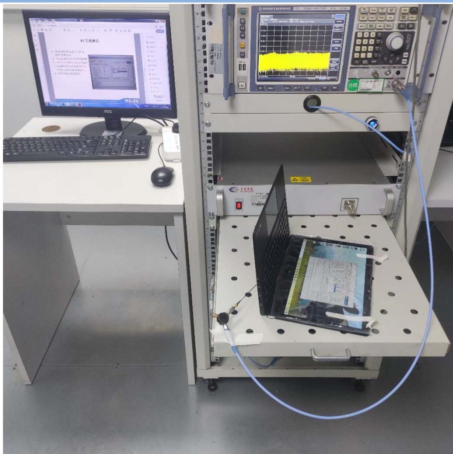
Conducted Test-BT3.0/BLE
