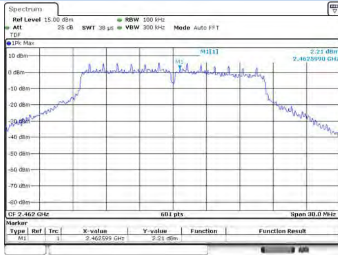
802.11g HIGH CHANNEL, Carrier level
