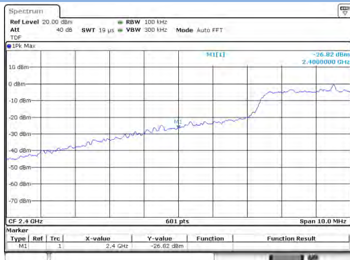
802.11ax-20 MHz (SU) LOW CHANNEL, Carrier level
