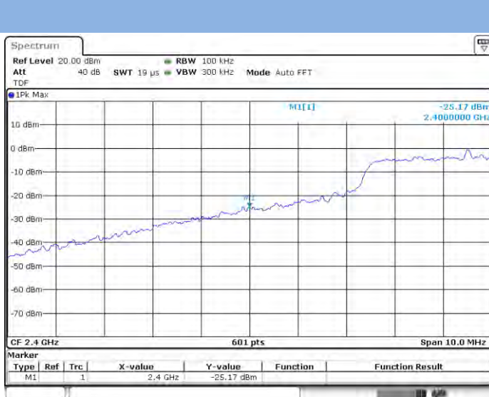
802.11ax-20 MHz (SU) LOW CHANNEL, Carrier level
