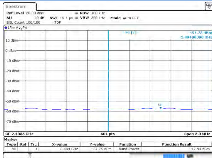
802.11ax-20 MHz (SU) HIGH CHANNEL, Reference level
