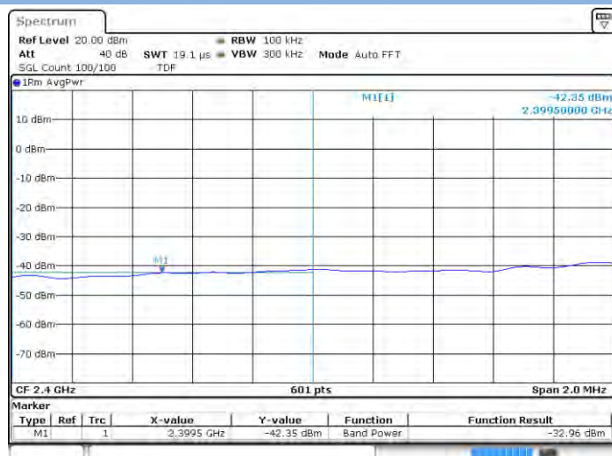
802.11ax-40 MHz (SU) LOW CHANNEL, Reference level
