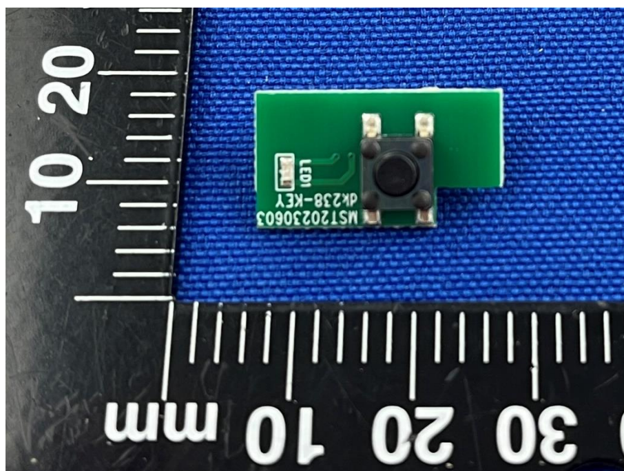
SECONDARY BOARD 6 TOP VIEW
