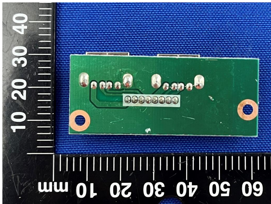
SECONDARY BOARD 5 REAR VIEW
