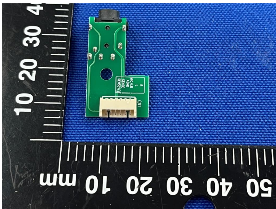
SECONDARY BOARD 7 TOP VIEW
