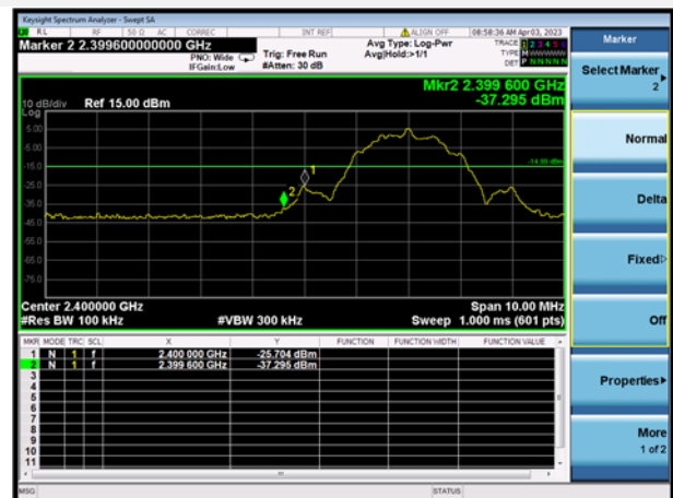
GFSK (BLE 2Mbps) LOW CHANNEL, BAND EDGE
