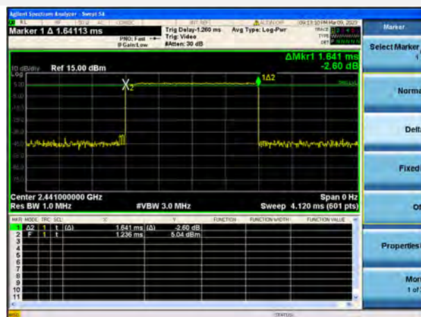
8-DPSK DH3
