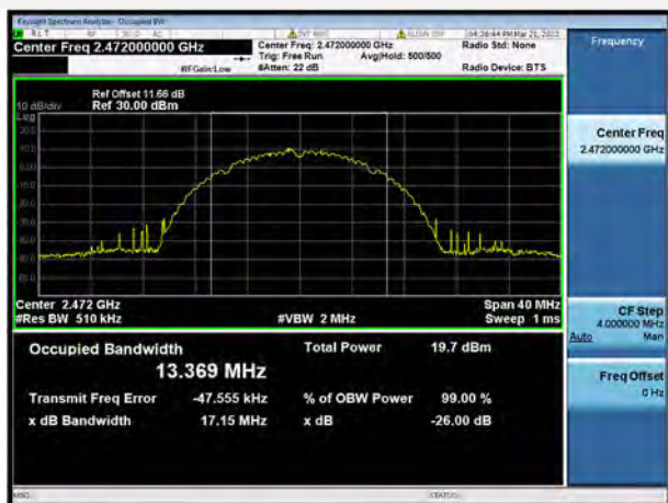
802.11b CHANNEL 13
