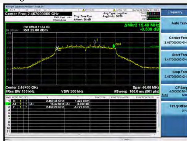
802.11g CHANNEL 12
