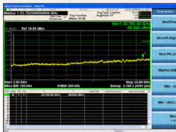
802.11b CHANNEL 6, SPURIOUS 2 GHz ~ 25 GHz
