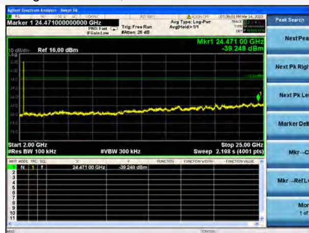
802.11g CHANNEL 1, SPURIOUS 2 GHz ~ 25 GHz
