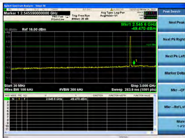
802.11b CHANNEL 13, SPURIOUS 30 MHz ~ 3 GHz
