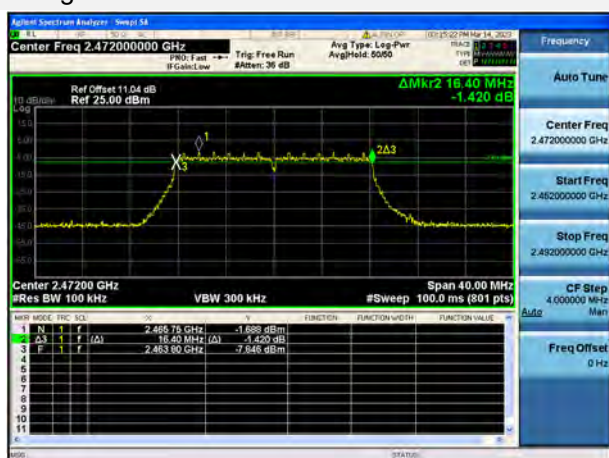
802.11g CHANNEL 13
