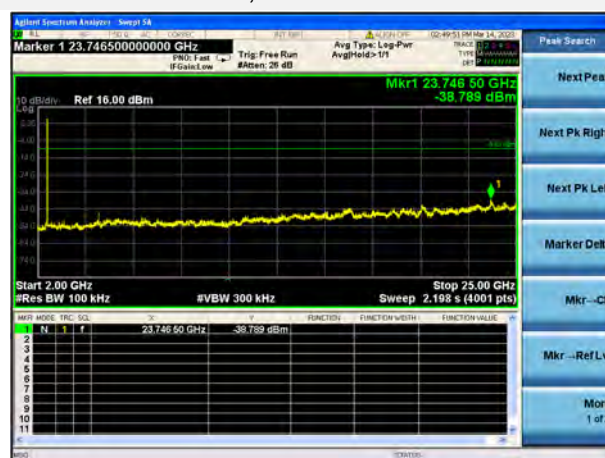
802.11b CHANNEL 11, SPURIOUS 2 GHz ~ 25 GHz
