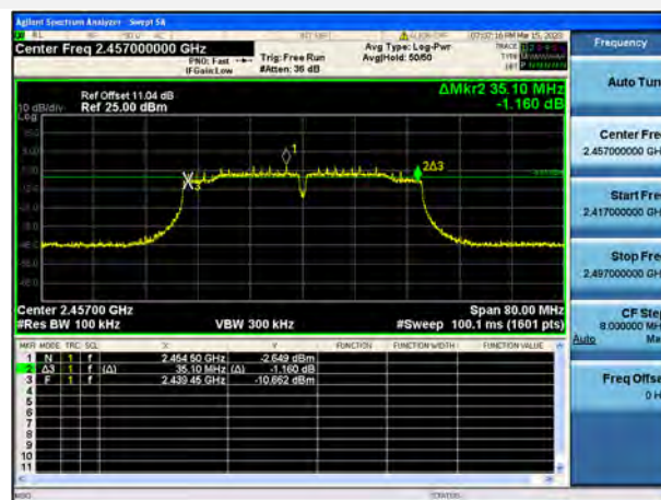
802.11n-40 MHz CHANNEL 10
