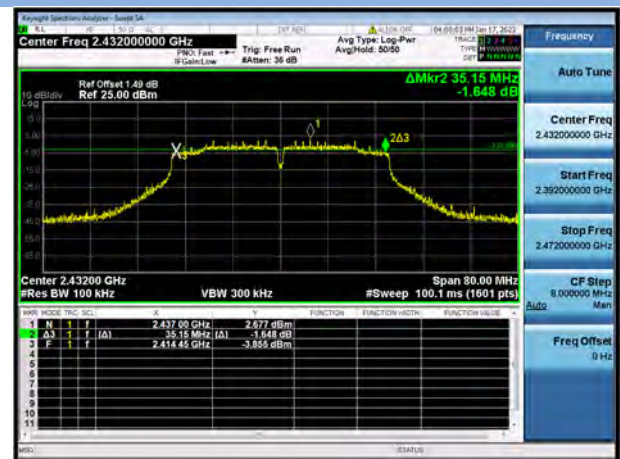
802.11n-40 MHz CHANNEL 5
