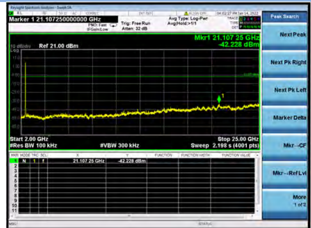
802.11g CHANNEL 6, SPURIOUS 2 GHz ~ 25 GHz
