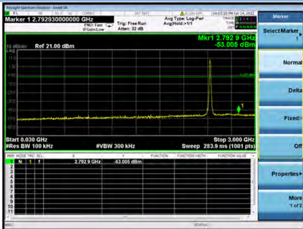
802.11g CHANNEL 6, SPURIOUS 30 MHz ~ 3 GHz
