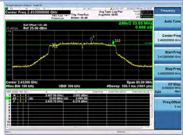
802.11ax-40 MHz(SU) CHANNEL 9
