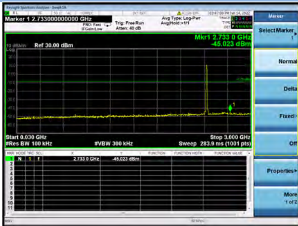
802.11b CHANNEL 6, SPURIOUS 30 MHz ~ 3 GHz
