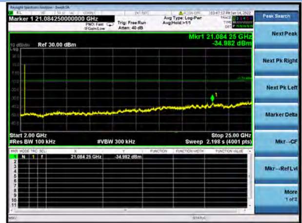
802.11b CHANNEL 6, SPURIOUS 2 GHz ~ 25 GHz
