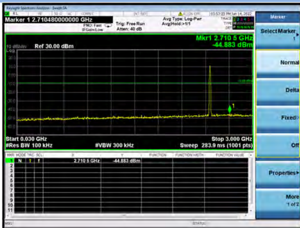
802.11b CHANNEL 11, SPURIOUS 30 MHz ~ 3 GHz
