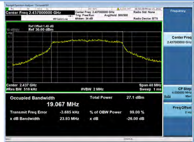
802.11ax-20 MHz(SU) CHANNEL 6
