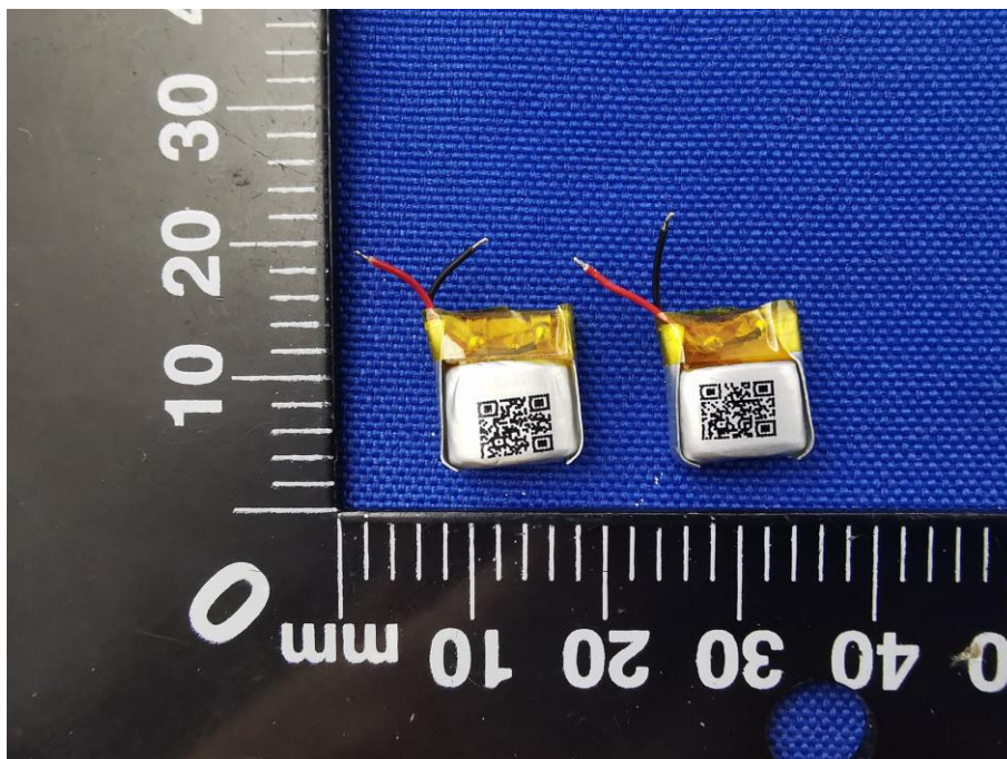
Battery Photo (REAR) (Model Name: ZWD541112)
