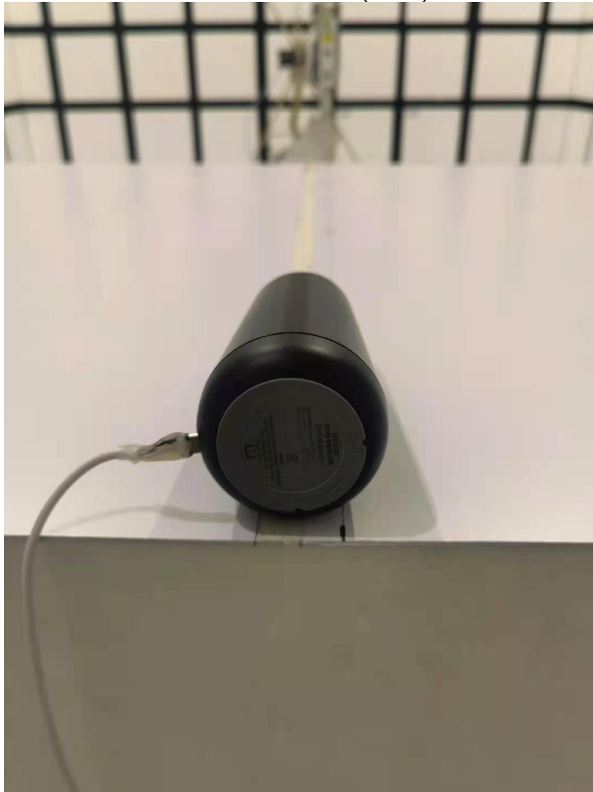
MEASUREMENT POSITION (X axis) for NFC
