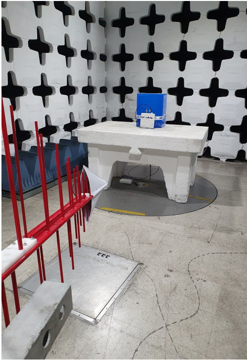
Radiated spurious emission test setup up to 1GHz.
