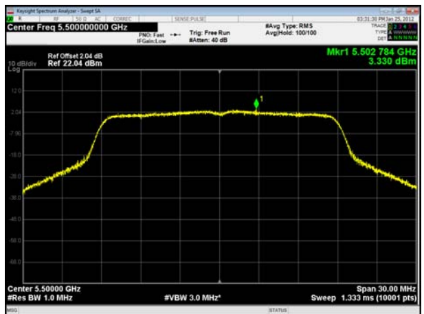
U-NII-2C, 802.11a, Channel No.: 100
