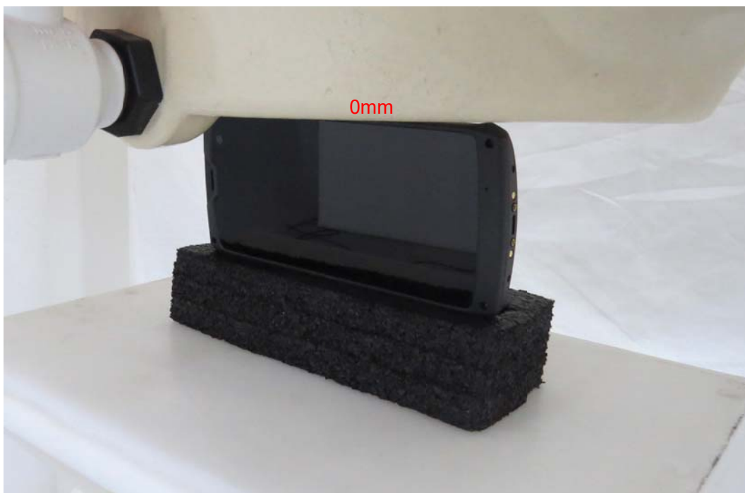
Picture 6: Right Side, the distance from handset to the bottom of the Phantom is 0mm
