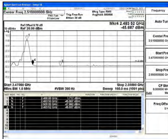
DH5_Ant1_High_2480_Peak
