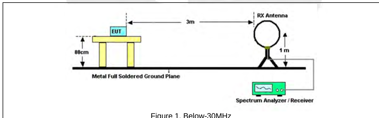
Figure 1. Below-30MHz
