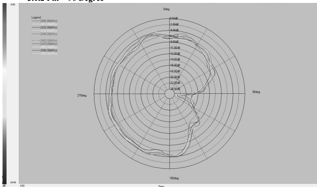
Fig 6. 2D Radiation Pattern Phi = 90 Degree 2400MHz to 2500MHz
