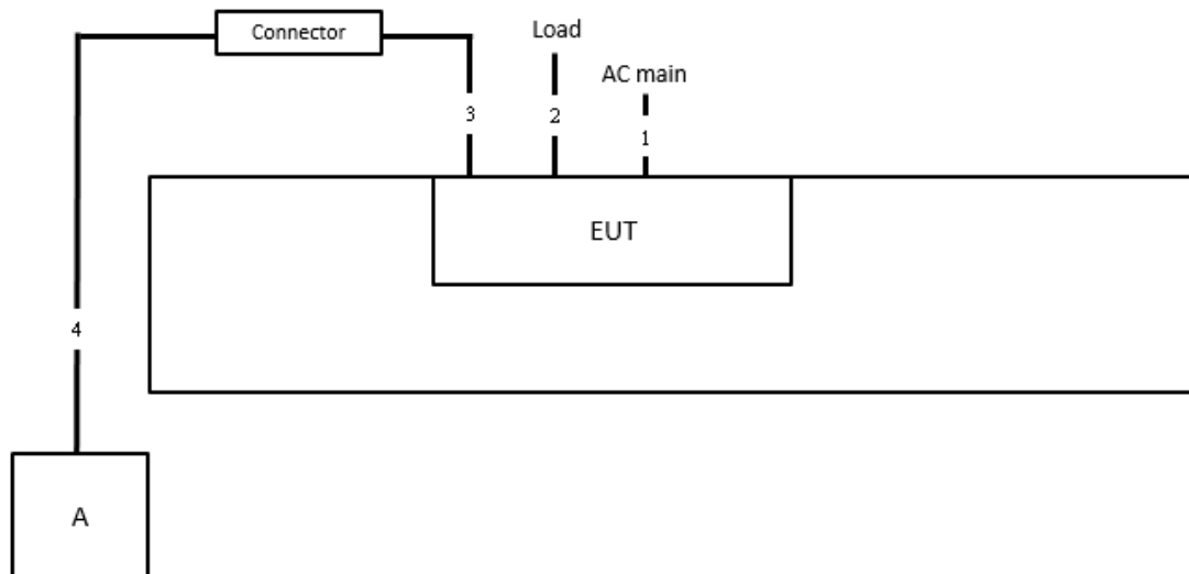
Test Setup Diagram - Radiated Test < 1GHz
