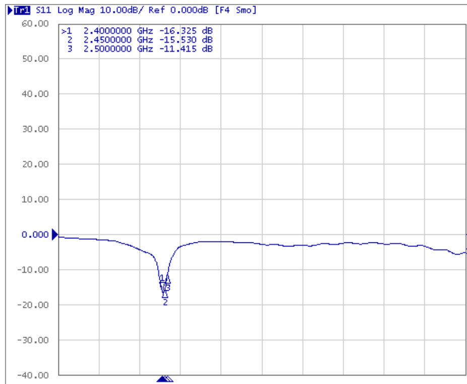
Figure 1 Return Loss
