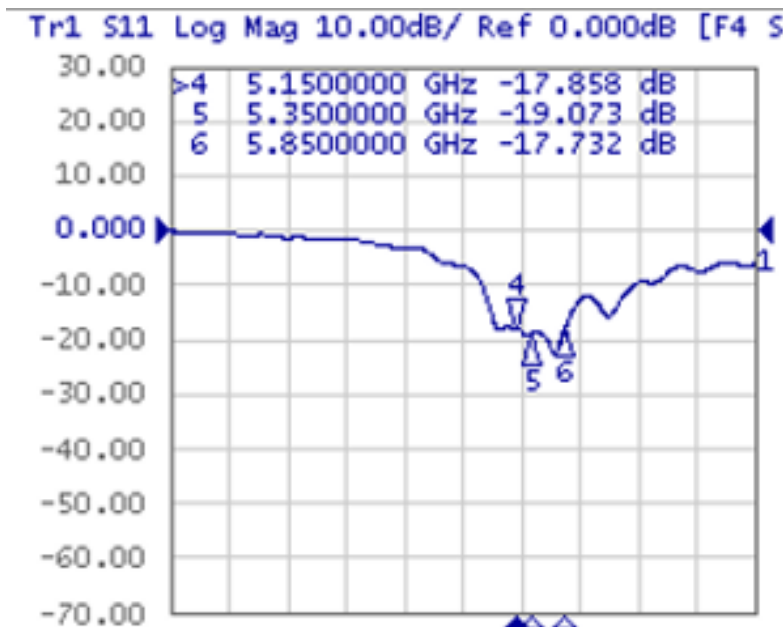
Figure 1 Return Loss
