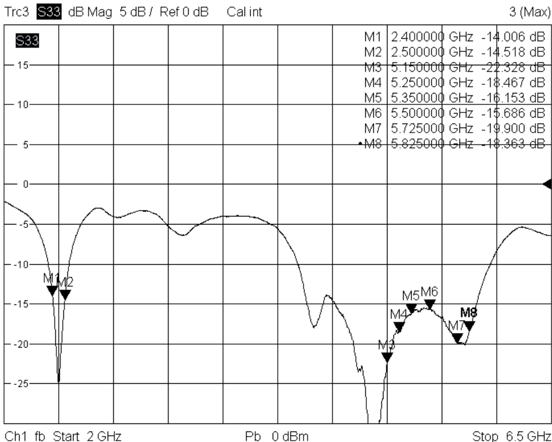
Figure 2 Return Loss
