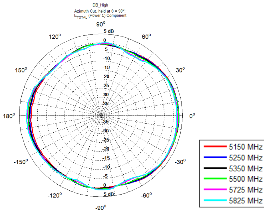
(A). Azimuth plane (XY plane) radiation pattern of 5GHz band
