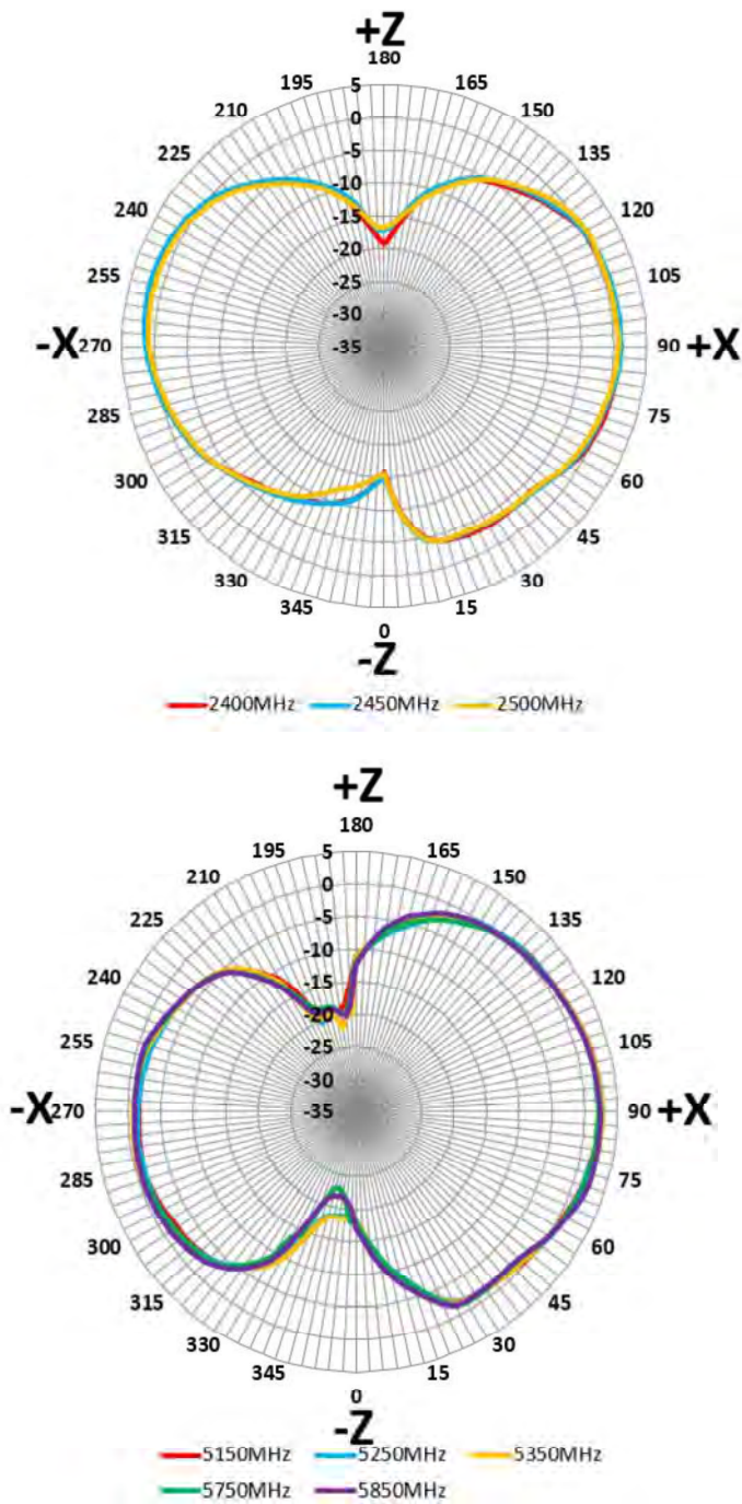
(B). Elevation 1 plane (XZ plane) radiation pattern
