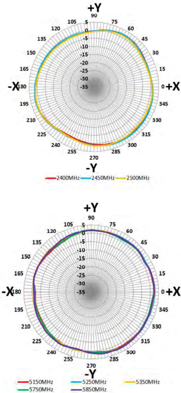
(A). Azimuth plane (XY plane) radiation pattern
