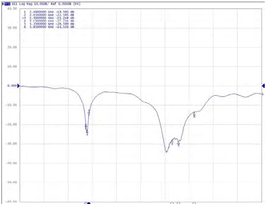
Figure 2 Return Loss
